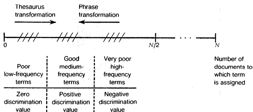
FIGURE 3. Term-Discrimination Model
